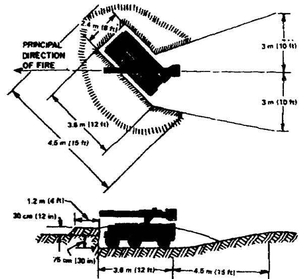
Figure 1-23. Emplacement for 106-mm rifle TOW missile.
